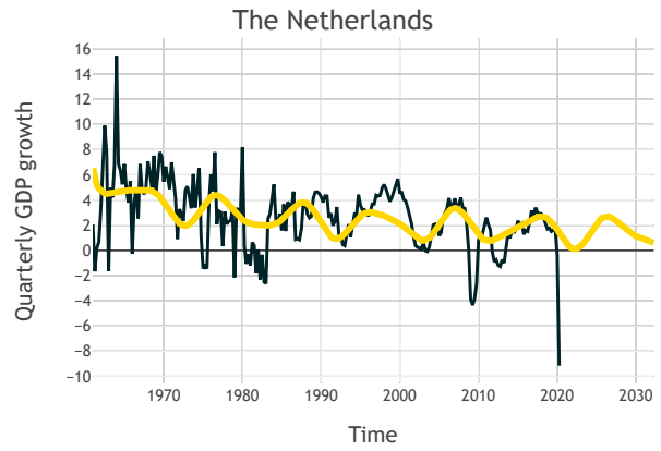
Figure 24: harmonic regression fit for The Netherlands.
